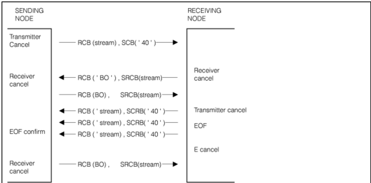
Figure 25. Sending Node Initiates Stream End
