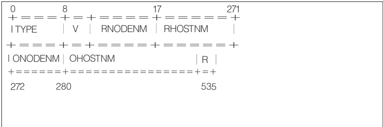
Figure 61. Format of an IPv6 NJE Control Record
