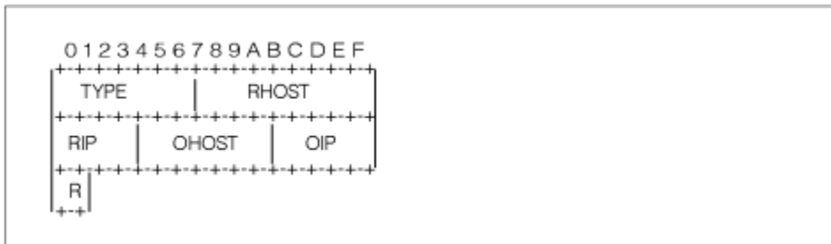
Figure 59. Format for the control record
