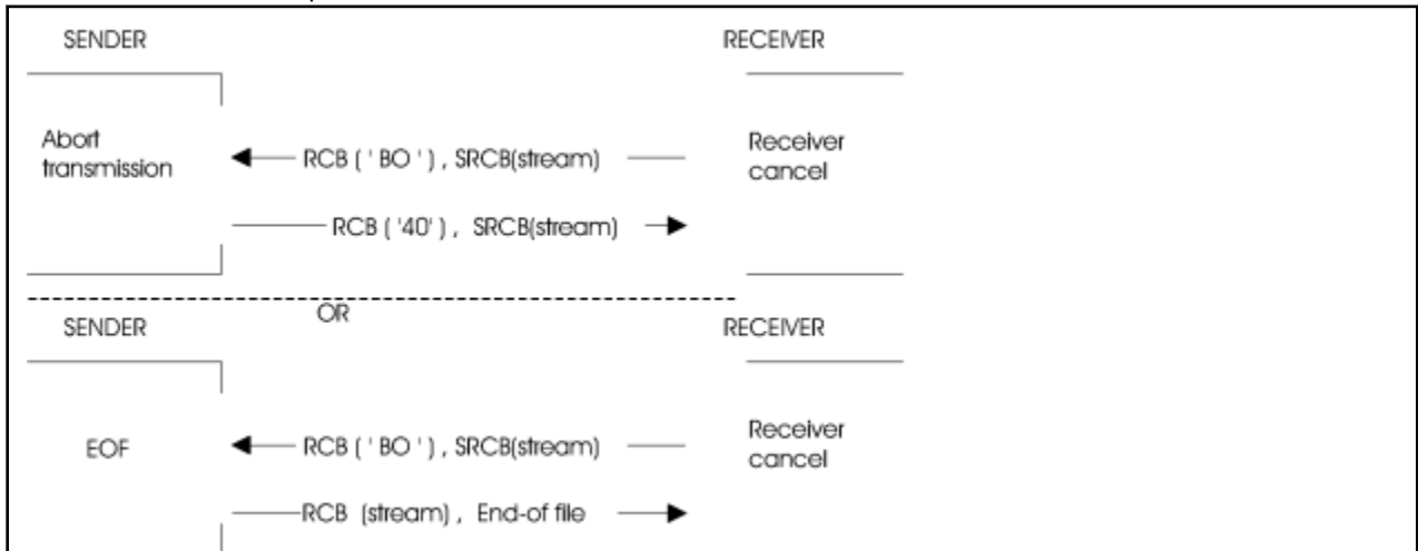
Figure 26. Receiving Node Initiates Stream End
