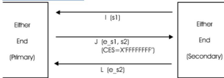
Figure 35. Secure connection (non-path manager trunk)
