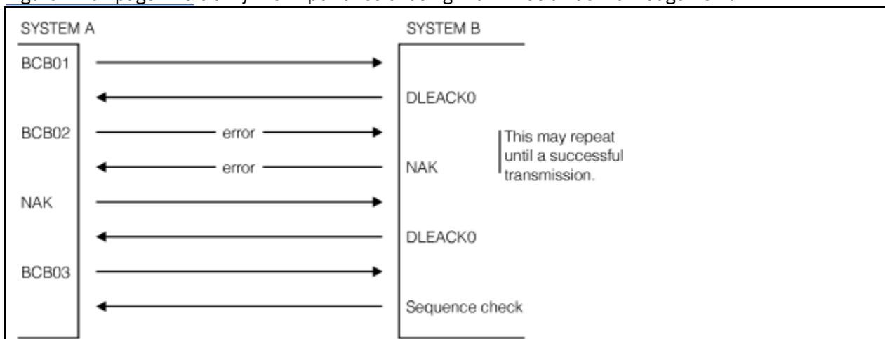
Figure 16. Results of Not Transmitting Null Records.
