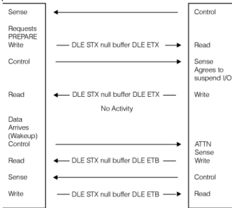
Figure 46. CTC Adapter Communication in PREPARE Mode
